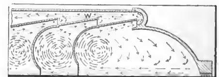
Fig. 5—Part section of Miller muffler
